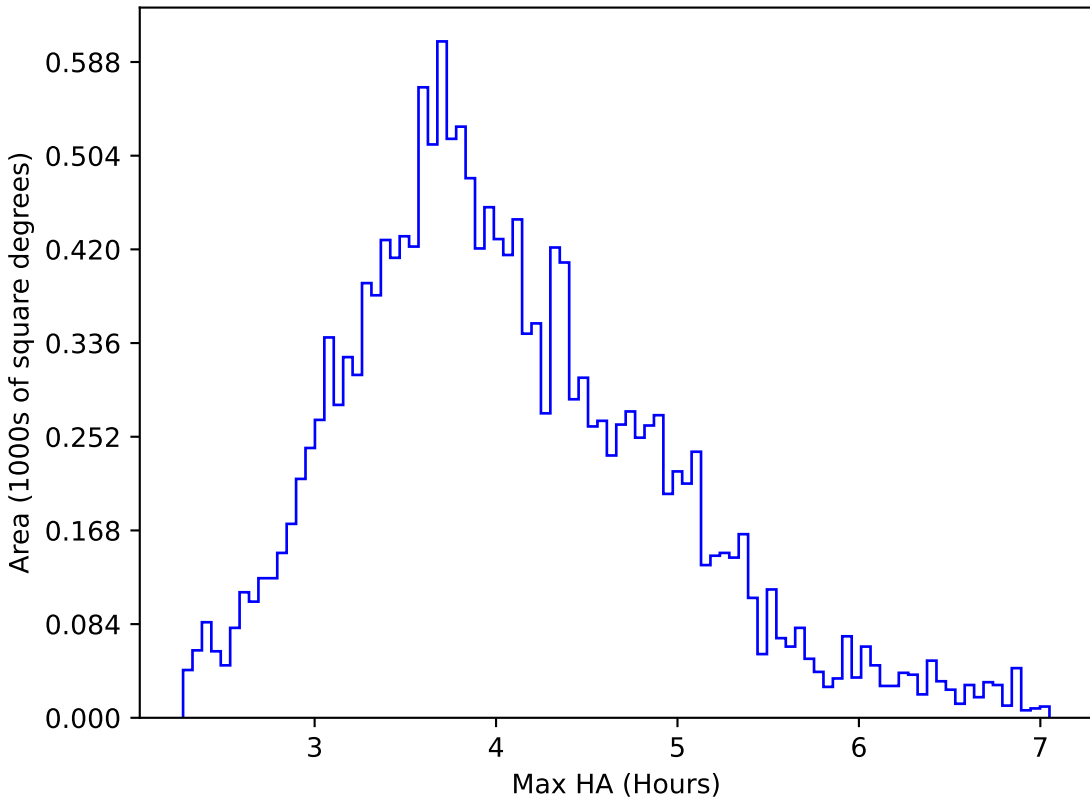
ddf_acor_sf20_lsf40_lsr50_v3.4_10yrs WFD g band: Max HA
