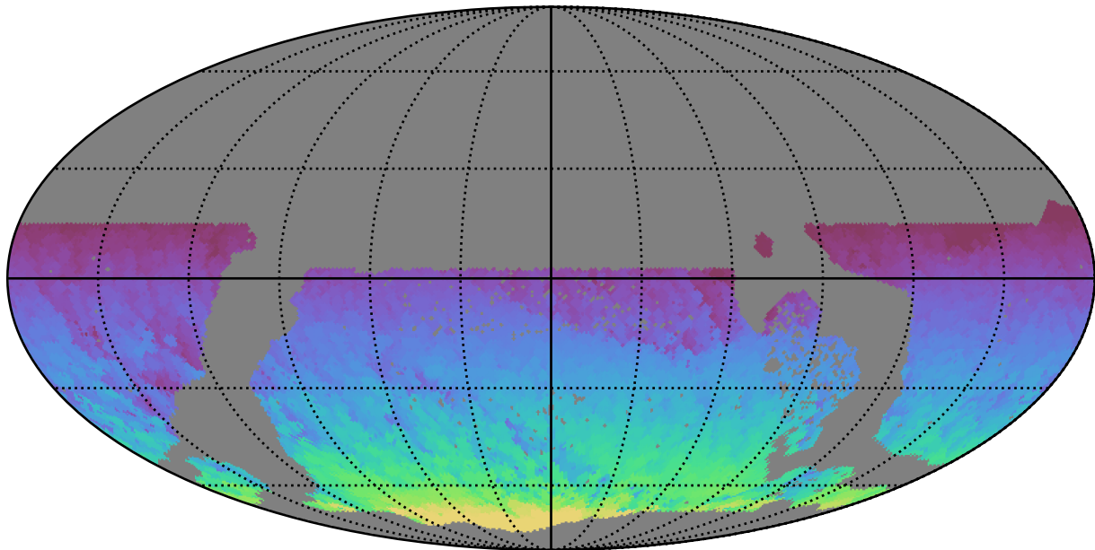
ddf_acor_sf20_lsf40_lsr50_v3.4_10yrs WFD all bands: Max HA
