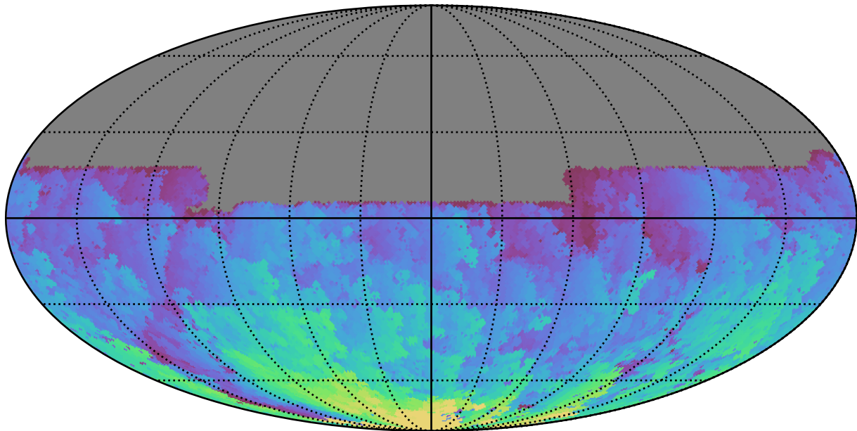
ddf_acor_sf20_lsf40_lsr50_v3.4_10yrs All sky u band: Max HA
