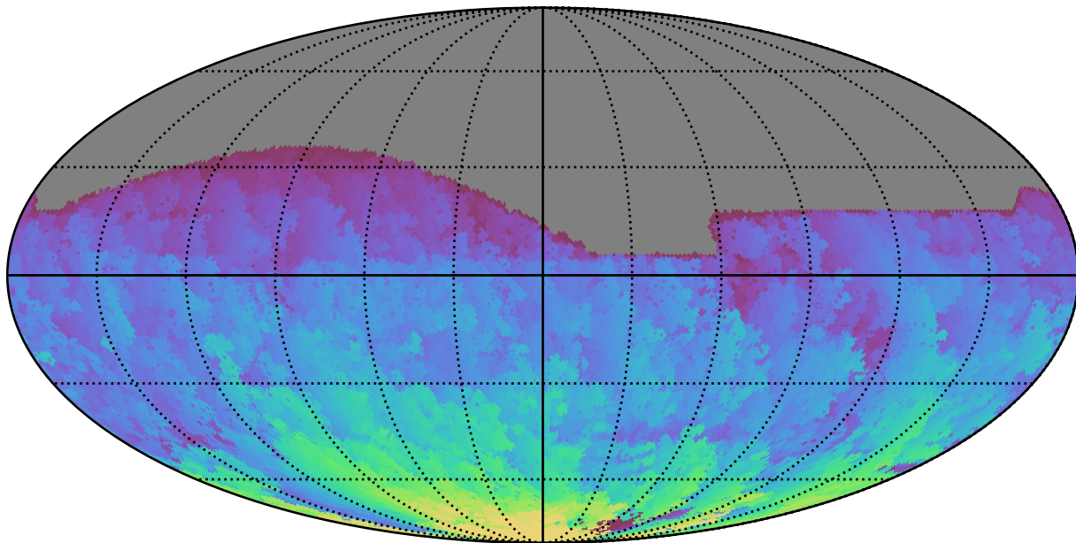
ddf_acor_sf20_lsf40_lsr50_v3.4_10yrs All sky r band: Max HA
