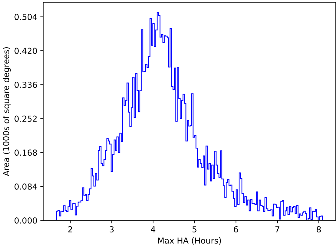
ddf_acor_sf20_ls40_lsr50_v3.4_10yrs All sky r band: Max HA
