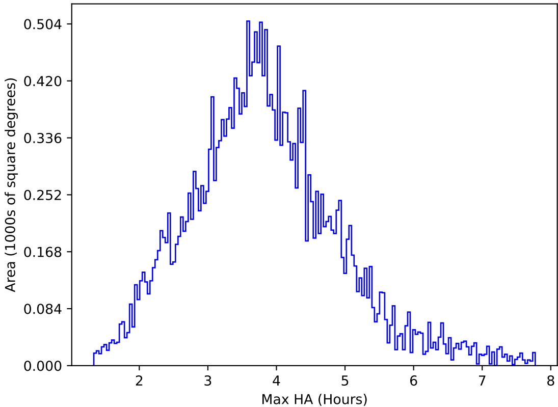
ddf_acor_sf20_lsf40_lsr50_v3.4_10yrs All sky g band: Max HA
