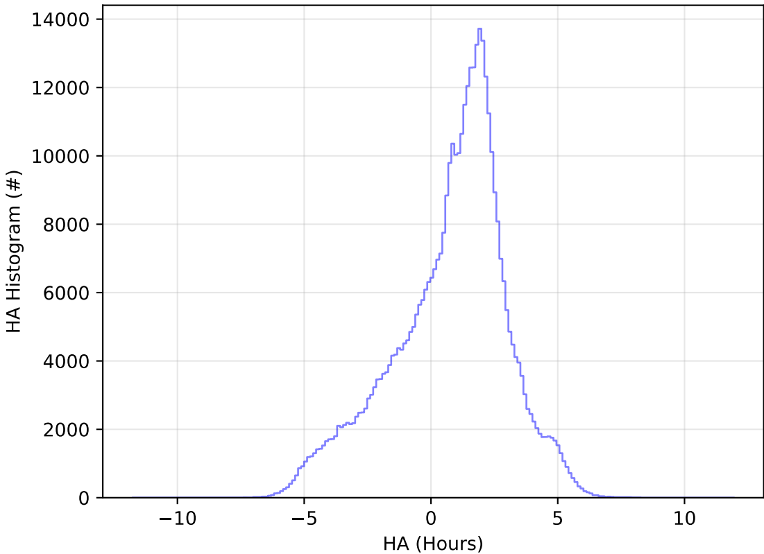
ddf_acor_sf20_lsf40_lsr50_v3.4_10yrs WFD z band: HA Histogram
