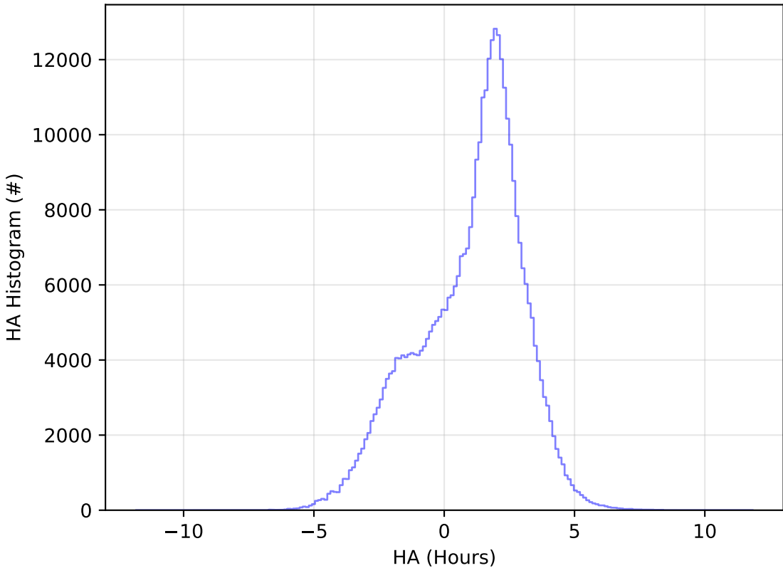
ddf_acor_sf20_lsf40_lsr50_v3.4_10yrs WFD y band: HA Histogram
