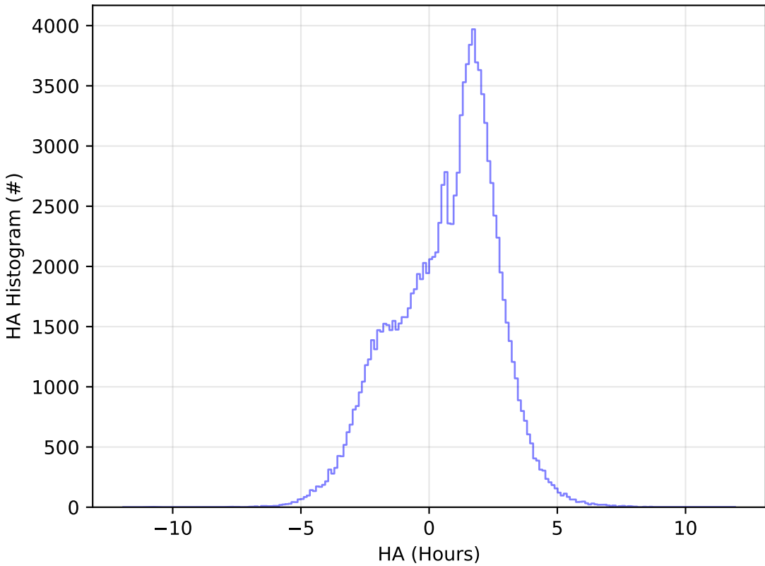
ddf_acor_sf20_lsf40_lsr50_v3.4_10yrs WFD u band: HA Histogram
