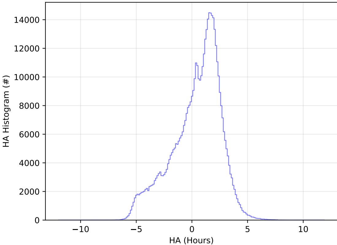
ddf_acor_sf20_lsf40_lsr50_v3.4_10yrs WFD r band: HA Histogram
