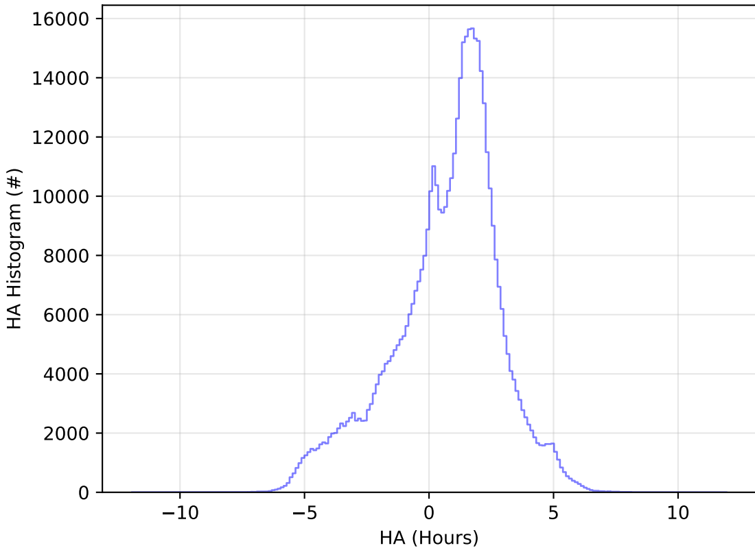
ddf_acor_sf20_lsf40_lsr50_v3.4_10yrs WFD i band: HA Histogram
