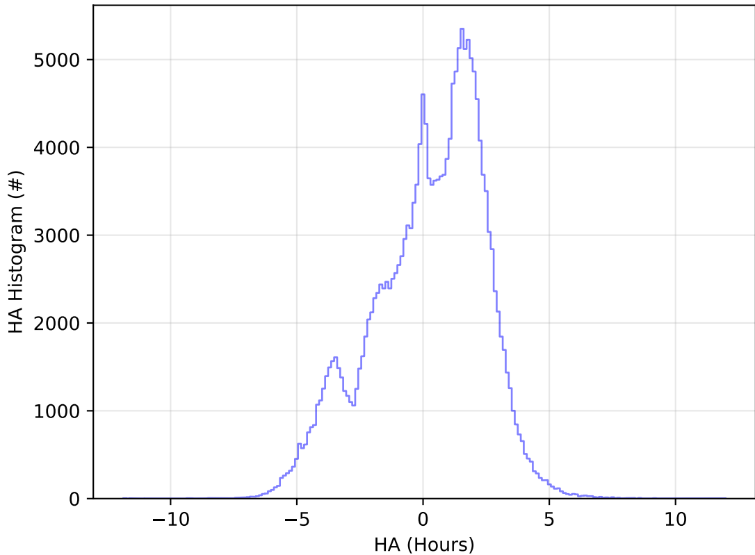
ddf_acor_sf20_lsf40_lsr50_v3.4_10yrs WFD g band: HA Histogram
