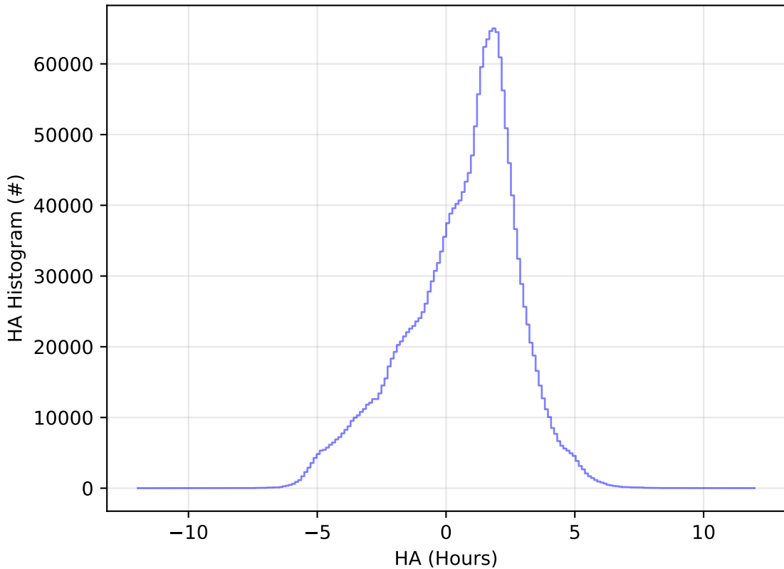
ddf_acor_sf20_lsf40_lsr50_v3.4_10yrs WFD all bands: HA Histogram
