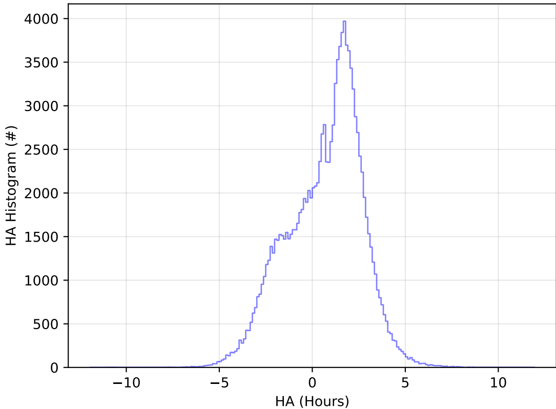
ddf_acor_sf20_lsf40_lsr50_v3.4_10yrs All sky u band: HA Histogram
