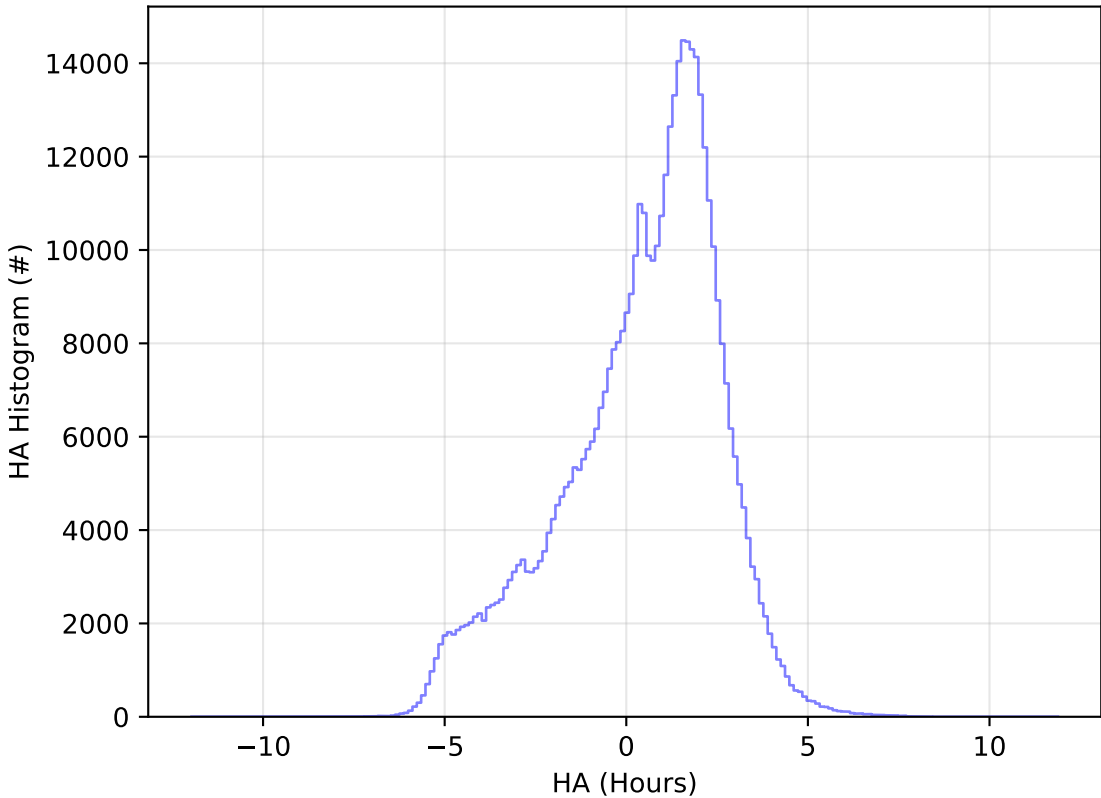
ddf_acor_sf20_lsf40_lsr50_v3.4_10yrs All sky r band: HA Histogram
