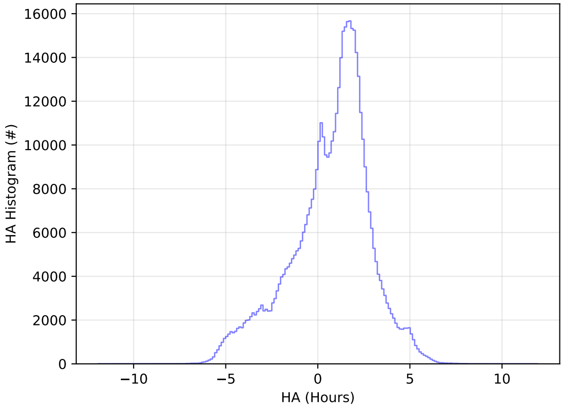
ddf_acor_sf20_lsf40_lsr50_v3.4_10yrs All sky i band: HA Histogram
