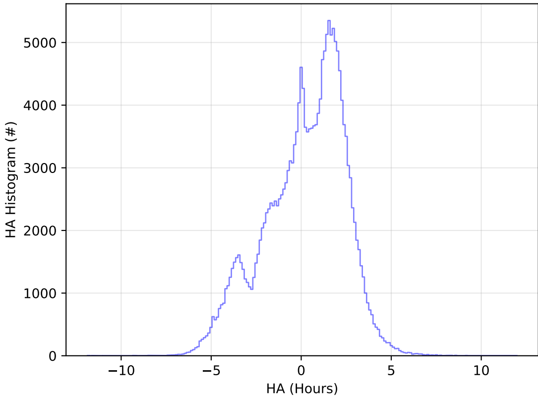
ddf_acor_sf20_lsf40_lsr50_v3.4_10yrs All sky g band: HA Histogram
