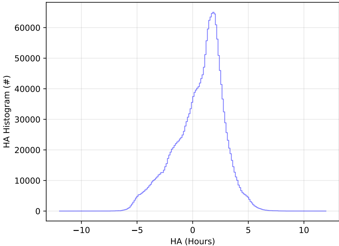
ddf_acor_sf20_lsf40_lsr50_v3.4_10yrs All sky all bands: HA Histogram
