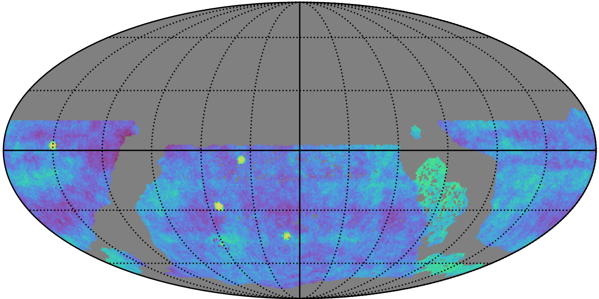
ddf_acor_sf20_lsf40_lsr50_v3.4_10yrs gri WFD: Fraction of visits in pairs (20-90 min)
