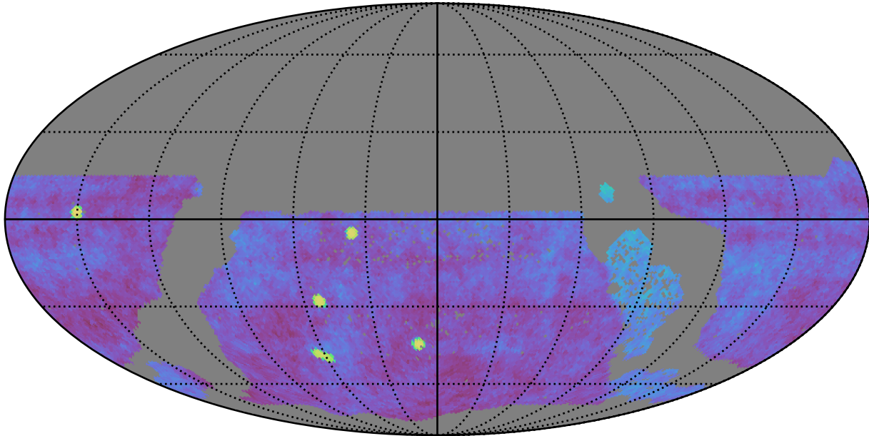
ddf_acor_sf20_lsf40_lsr50_v3.4_10yrs gri WFD: Fraction of visits in pairs (10-60 min)
