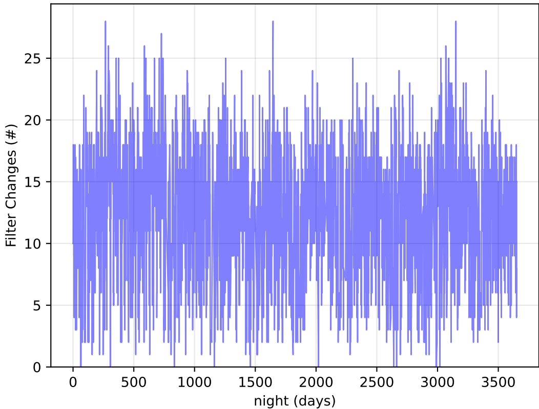
ddf_acor_sf20_Isf40_Isr50_v3.4_10yrs Per Night: Filter Changes
