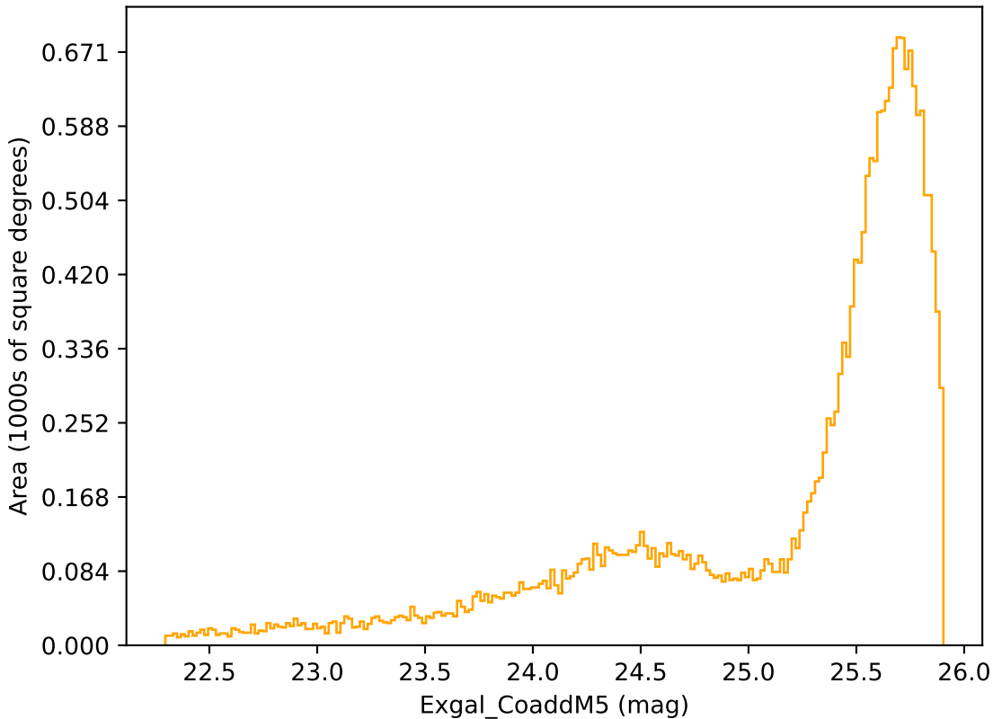
ddf_acor_sf20_lsf40_lsr50_v3.4_10yrs Yr 1 r band: Exgal_CoaddM5
