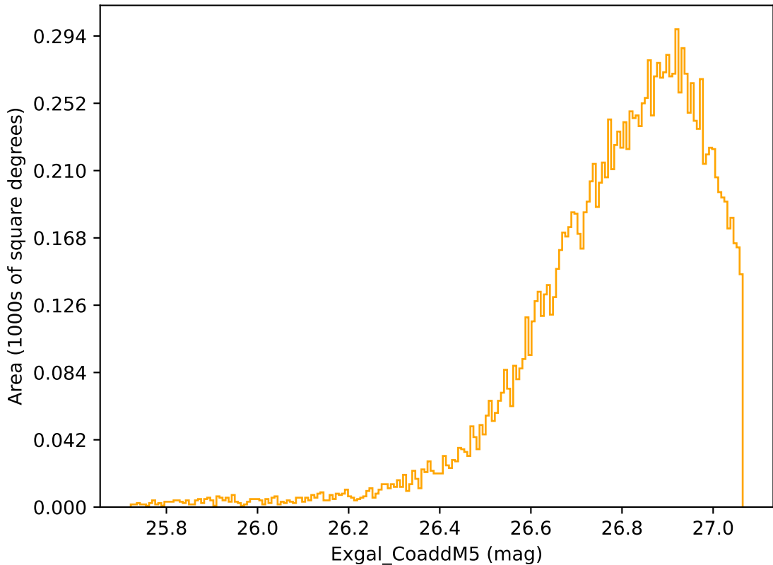
ddf_acor_sf20_lsf40_lsr50_v3.4_10yrs WFD r band: Exgal_CoaddM5
