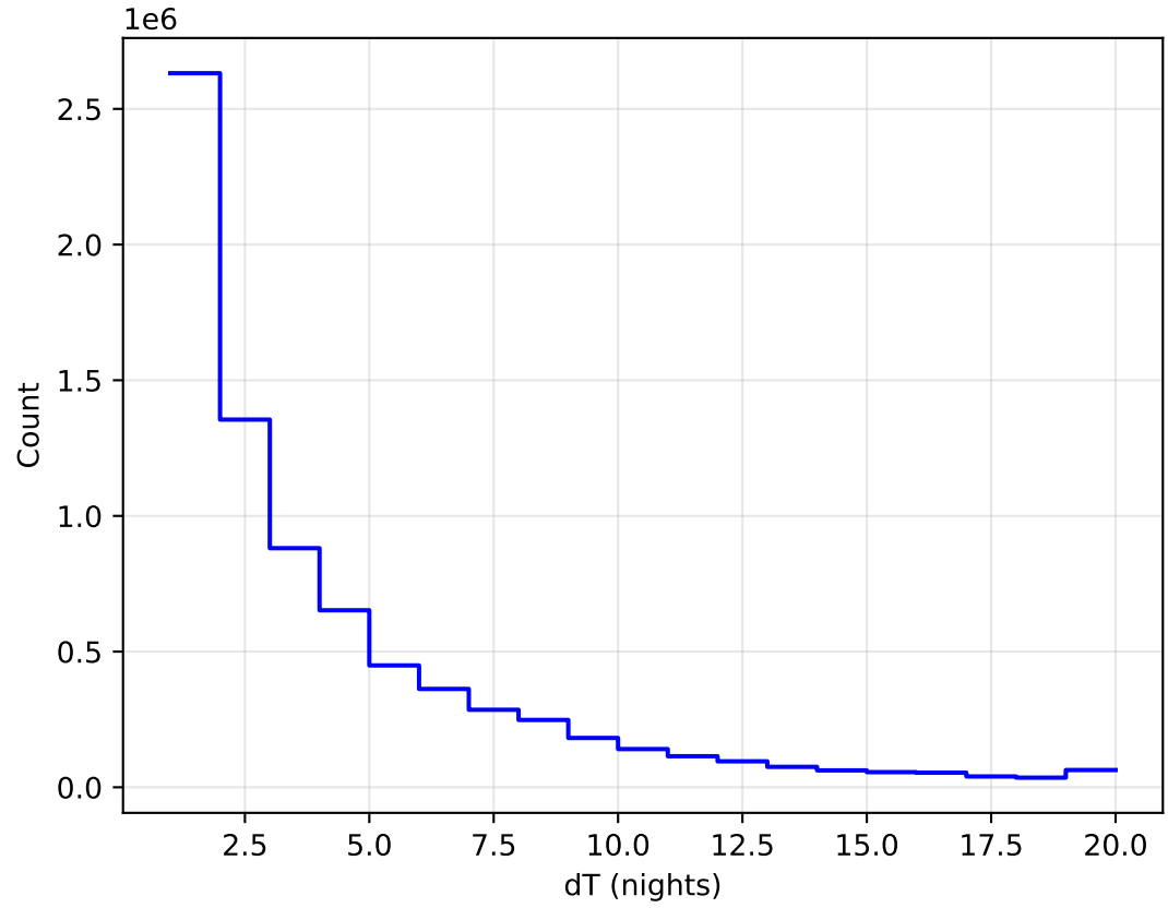
ddf_acor_sf20_lsf40_lsr50_v3.4_10yrs WFD all bands: DeltaNight Histogram
