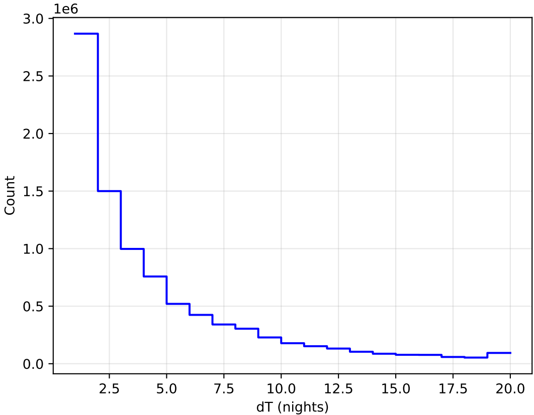
ddf_acor_sf20_lsf40_lsr50_v3.4_10yrs All sky all bands: DeltaNight Histogram
