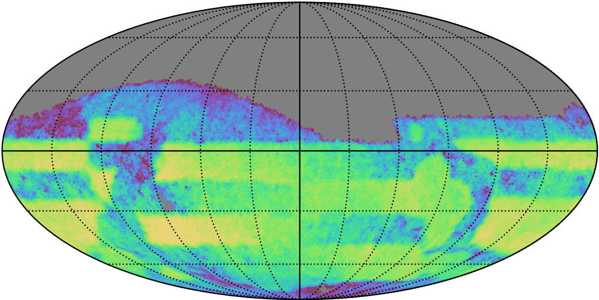
ddf_acor_sf20_lsf40_lsr50_v3.4_10yrs Yr 3-4 i band: CoaddM5
