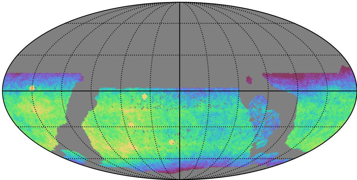
ddf_acor_sf20_lsf40_lsr50_v3.4_10yrs WFD z band: CoaddM5
