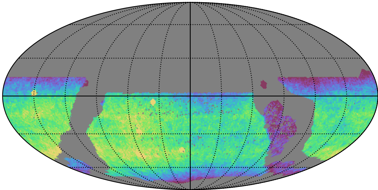
ddf_acor_sf20_lsf40_lsr50_v3.4_10yrs WFD y band: CoaddM5
