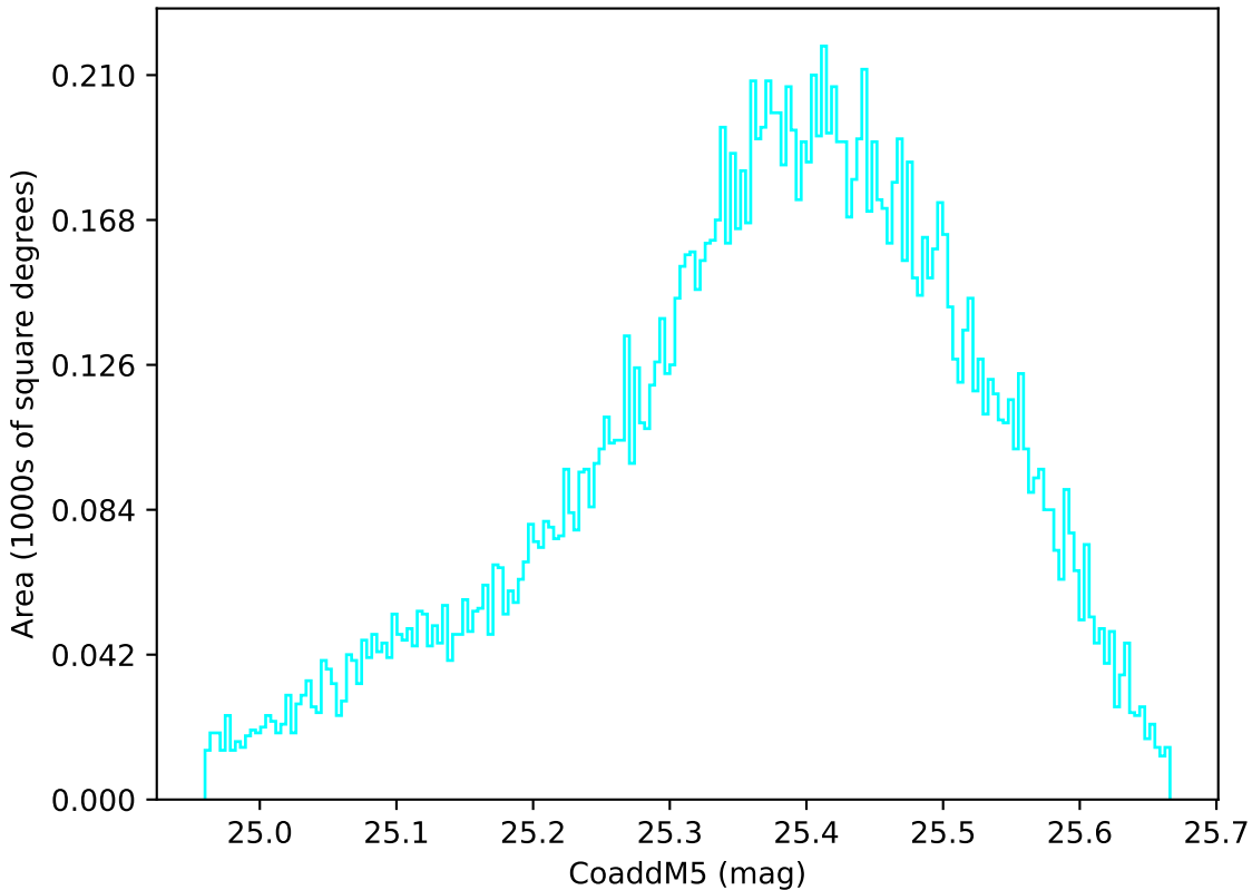
ddf_acor_sf20_lsf40_lsr50_v3.4_10yrs WFD u band: CoaddM5
