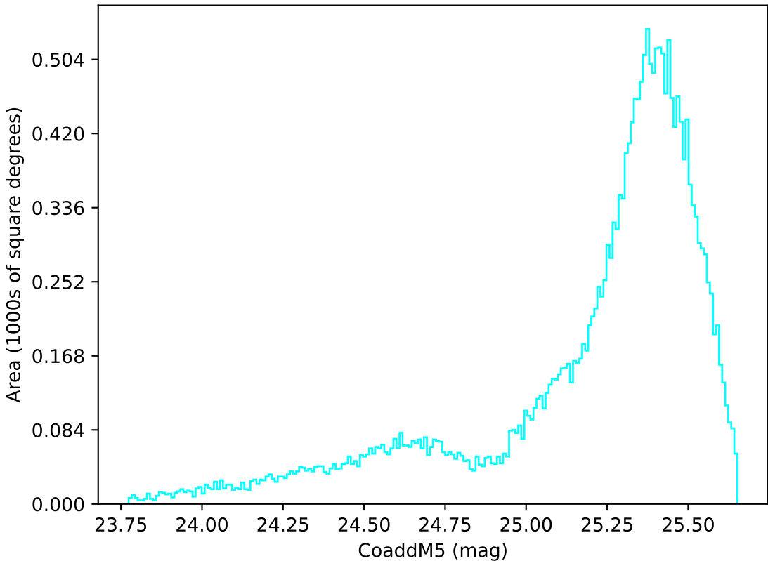
ddf_acor_sf20_lsf40_lsr50_v3.4_10yrs All sky u band: CoaddM5
