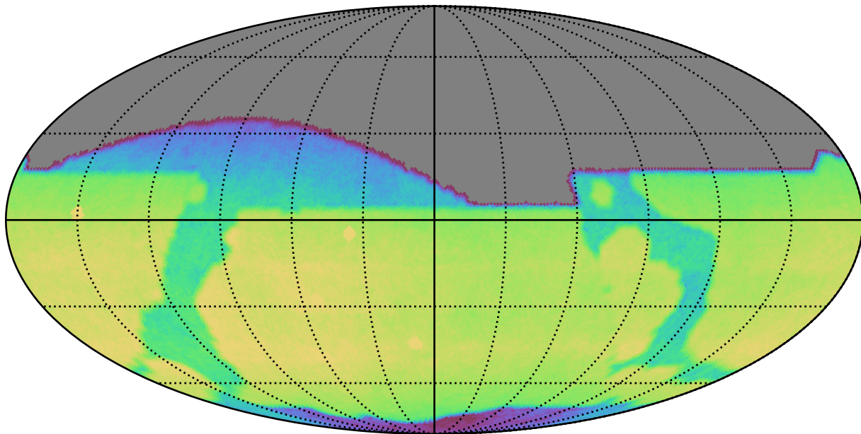
ddf_acor_sf20_lsf40_lsr50_v3.4_10yrs All sky r band: CoaddM5
