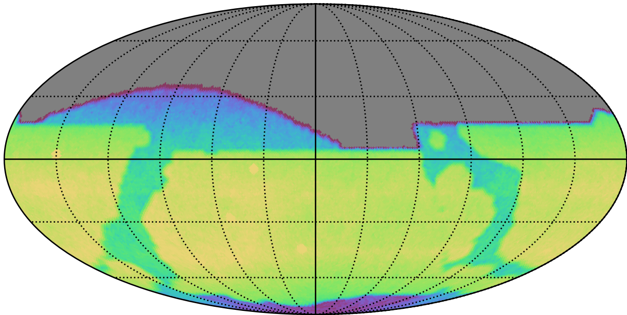
ddf_acor_sf20_lsf40_lsr50_v3.4_10yrs All sky i band: CoaddM5
