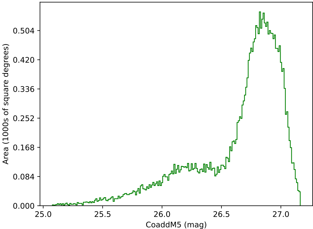
ddf_acor_sf20_lsf40_lsr50_v3.4_10yrs All sky g band: CoaddM5
