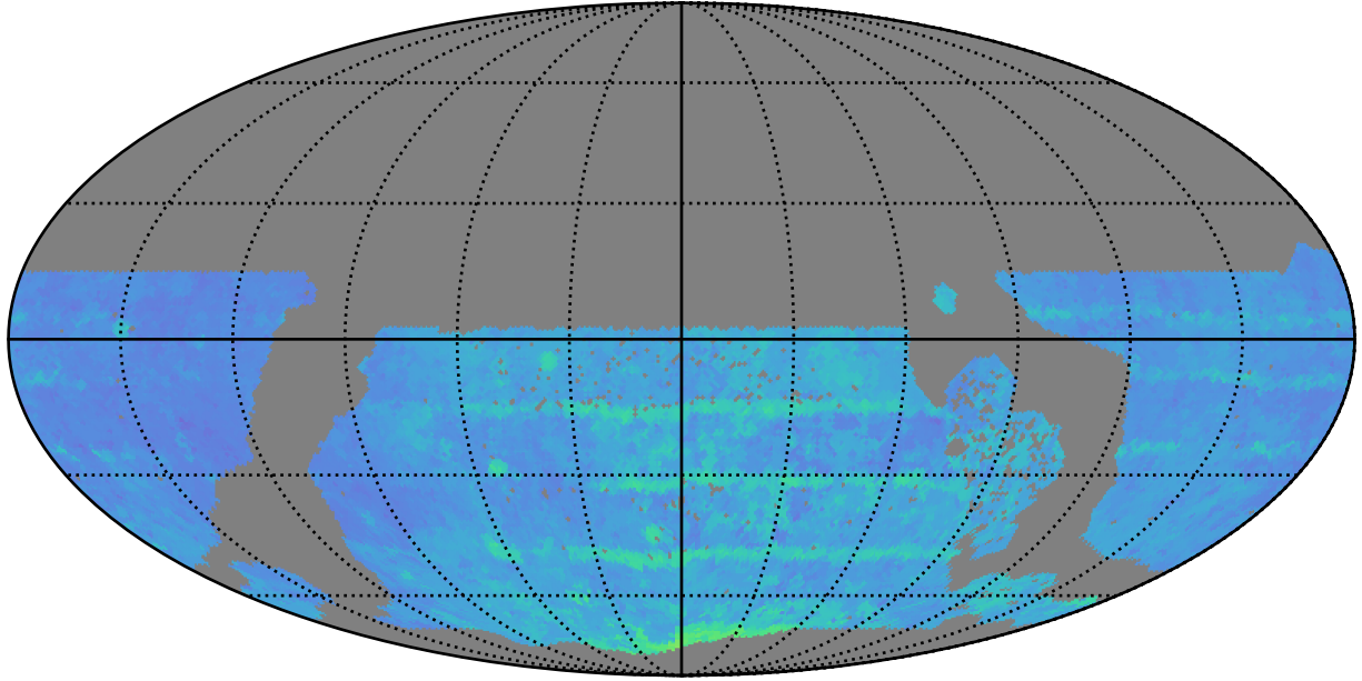
ddf_acor_sf20_lsf40_lsr50_v3.4_10yrs WFD z band: 80thPercentile Season Length
