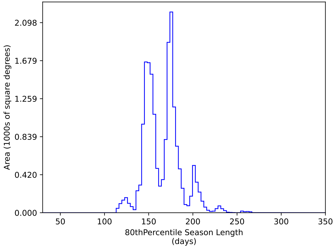
ddf_acor_sf20_lsf40_lsr50_v3.4_10yrs WFD y band: 80thPercentile Season Length
