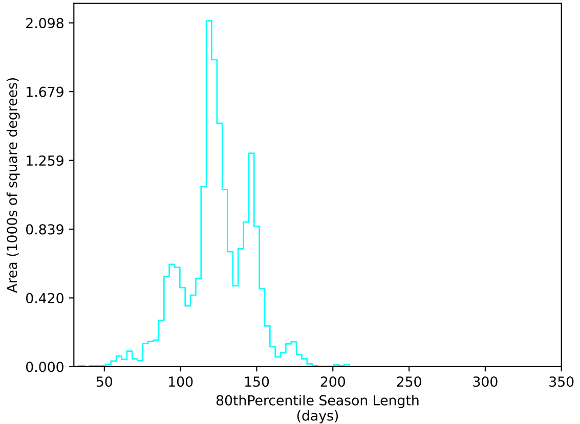
ddf_acor_sf20_lsf40_lsr50_v3.4_10yrs WFD u band: 80thPercentile Season Length
