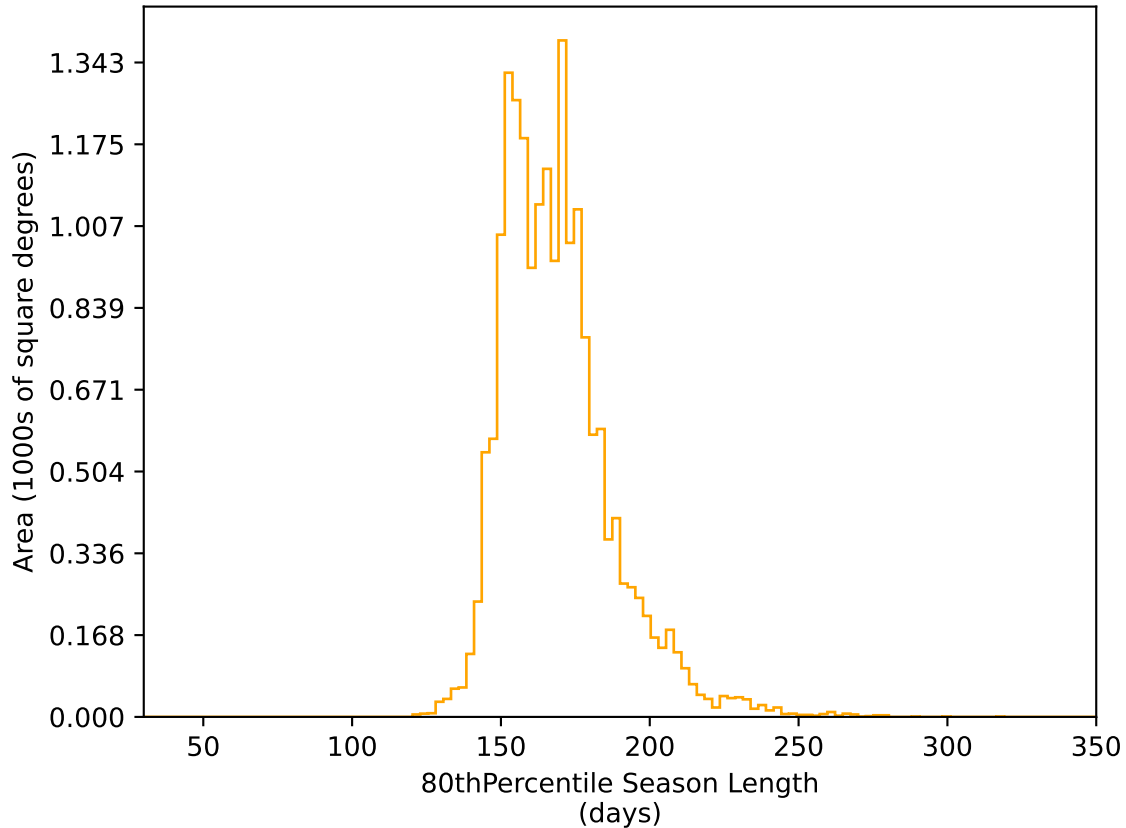
ddf_acor_sf20_lsf40_lsr50_v3.4_10yrs WFD r band: 80thPercentile Season Length
