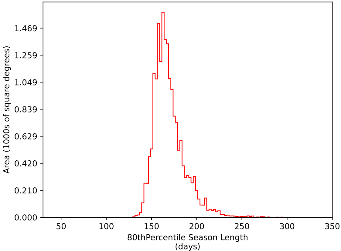
ddf_acor_sf20_lsf40_lsr50_v3.4_10yrs WFD i band: 80thPercentile Season Length
