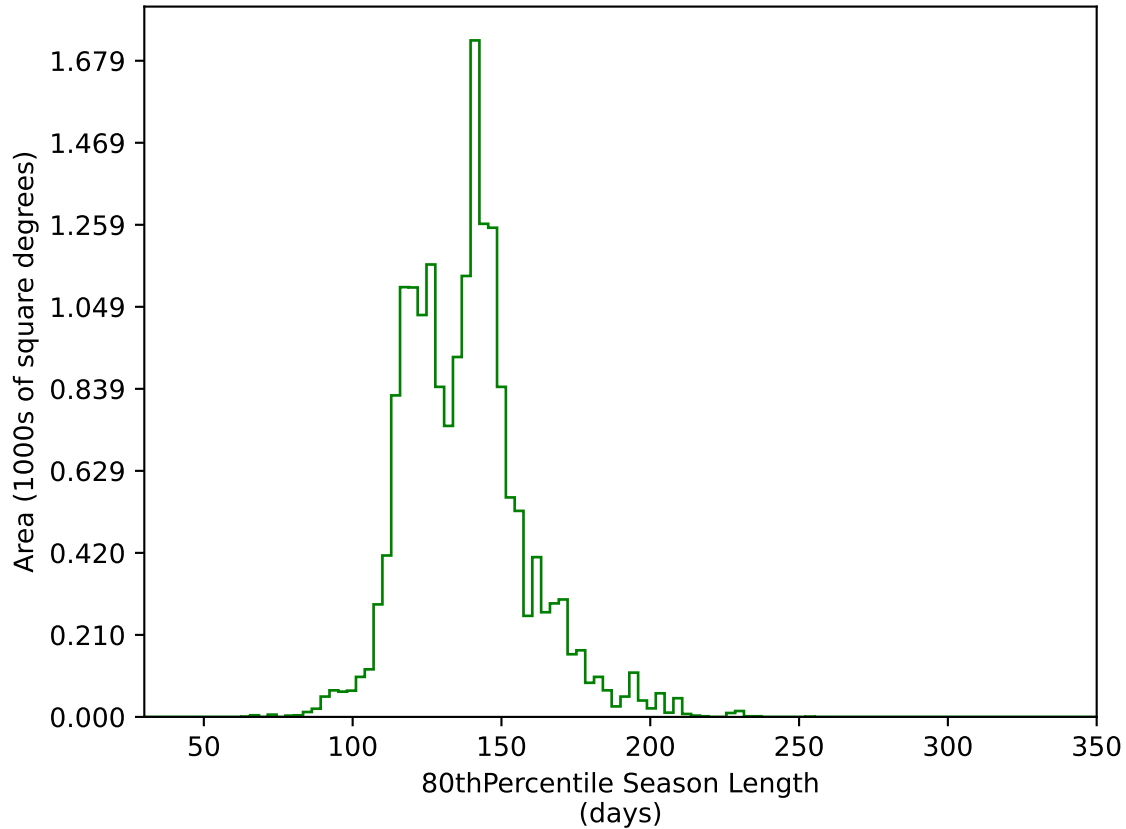
ddf_acor_sf20_lsf40_lsr50_v3.4_10yrs WFD g band: 80thPercentile Season Length
