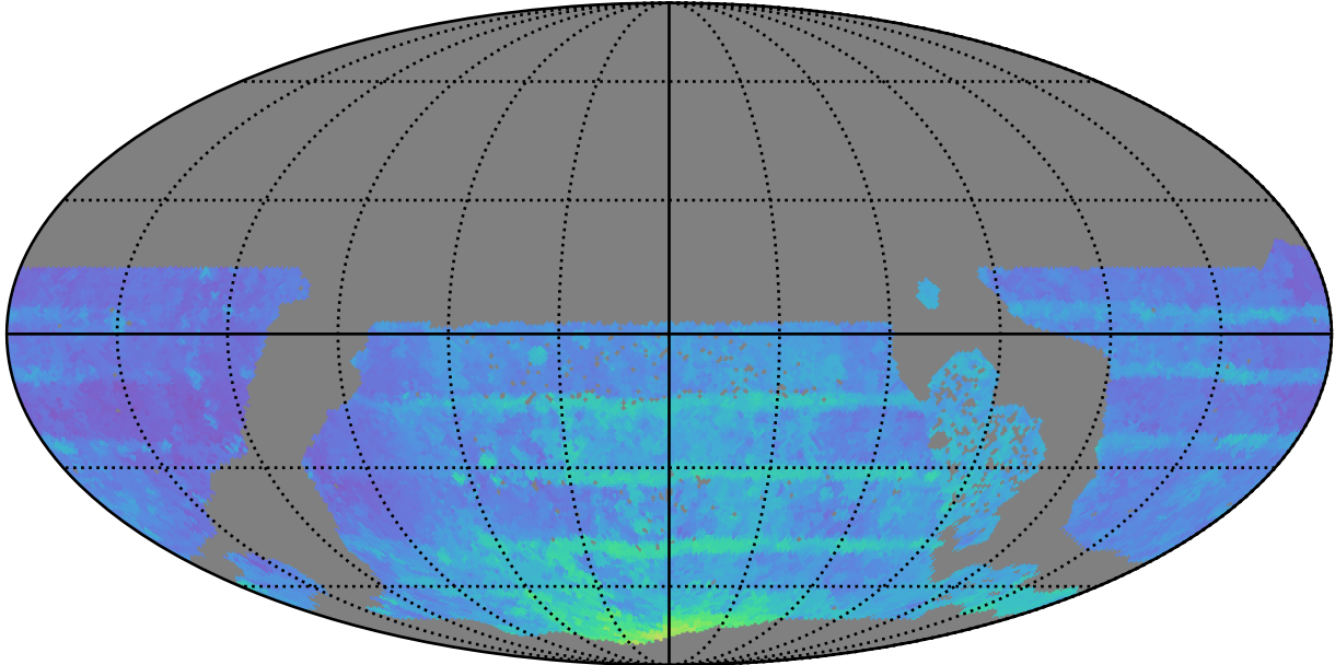
ddf_acor_sf20_lsf40_lsr50_v3.4_10yrs WFD all bands: 80thPercentile Season Length
