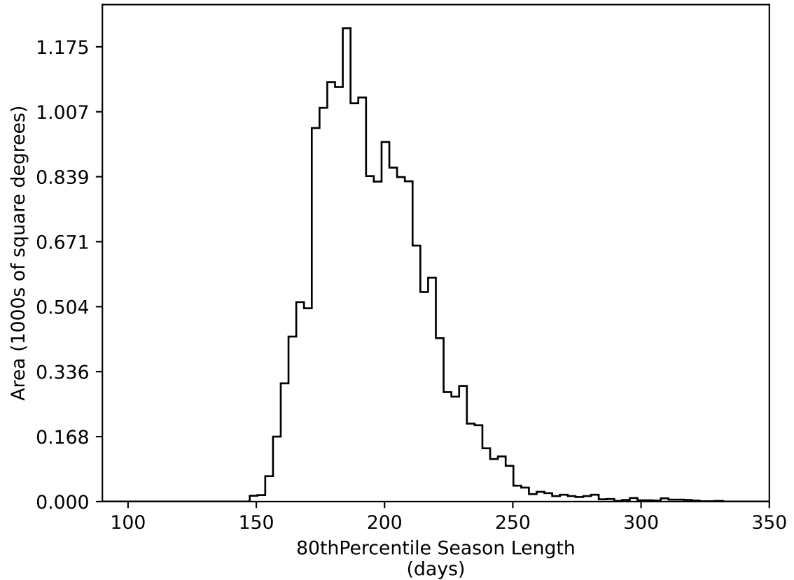
ddf_acor_sf20_lsf40_lsr50_v3.4_10yrs WFD all bands: 80thPercentile Season Length
