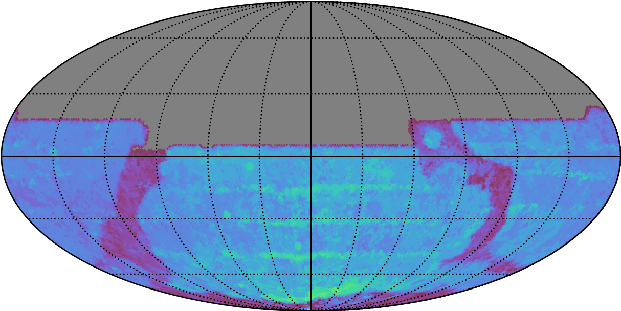
ddf_acor_sf20_lsf40_lsr50_v3.4_10yrs All sky y band: 80thPercentile Season Length
