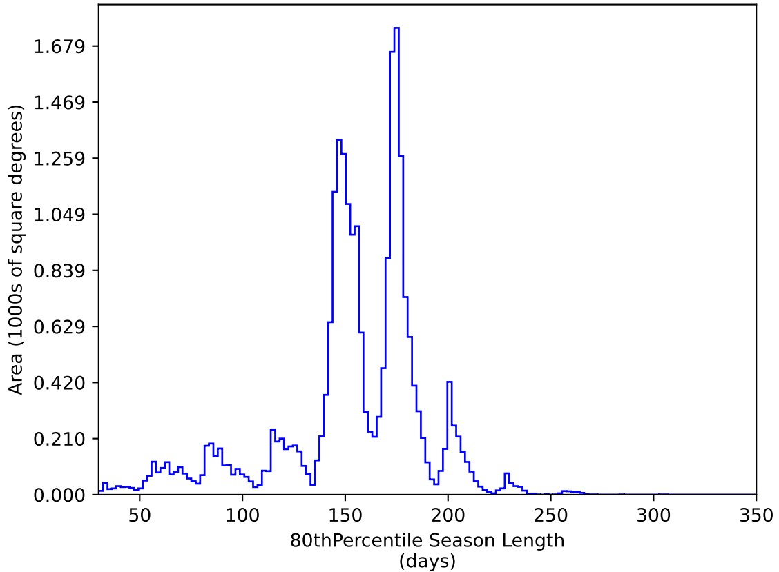
ddf_acor_sf20_lsf40_lsr50_v3.4_10yrs All sky y band: 80thPercentile Season Length
