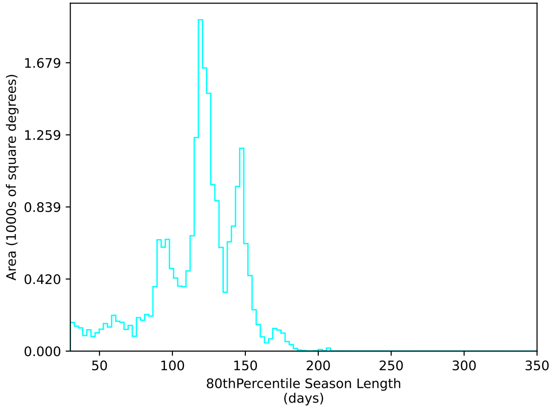
ddf_acor_sf20_lsf40_lsr50_v3.4_10yrs All sky u band: 80thPercentile Season Length
