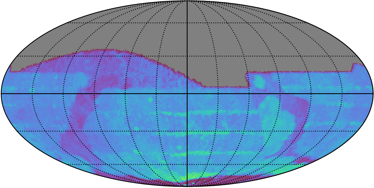
ddf_acor_sf20_lsf40_lsr50_v3.4_10yrs All sky r band: 80thPercentile Season Length
