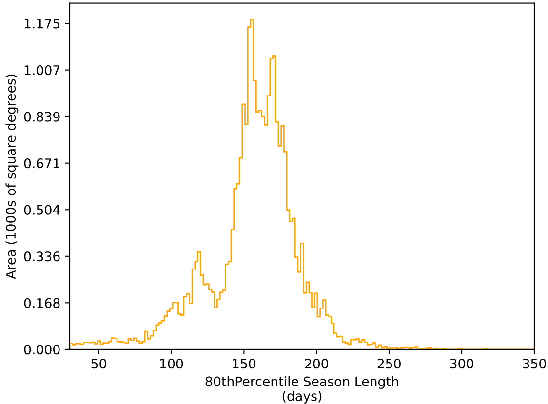
ddf_acor_sf20_lsf40_lsr50_v3.4_10yrs All sky r band: 80thPercentile Season Length
