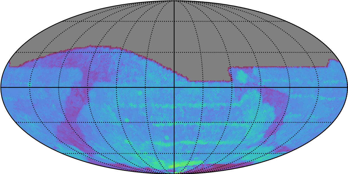
ddf_acor_sf20_lsf40_lsr50_v3.4_10yrs All sky i band: 80thPercentile Season Length
