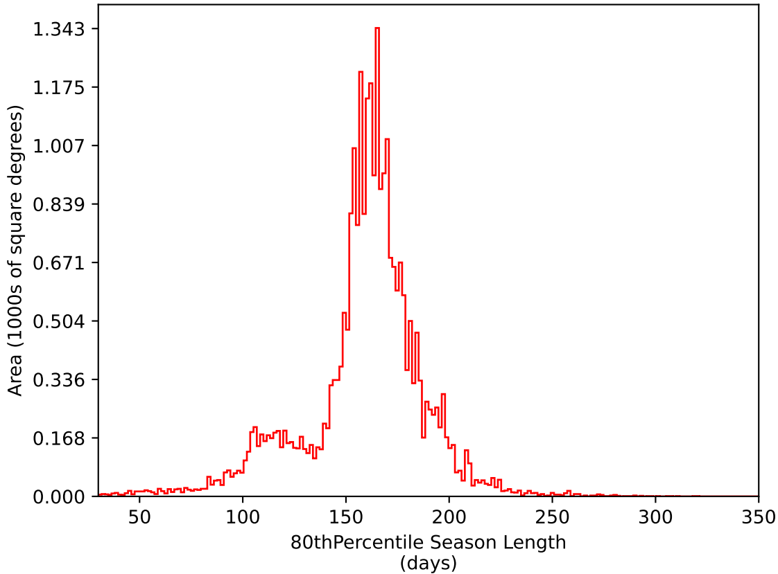
ddf_acor_sf20_lsf40_lsr50_v3.4_10yrs All sky i band: 80thPercentile Season Length
