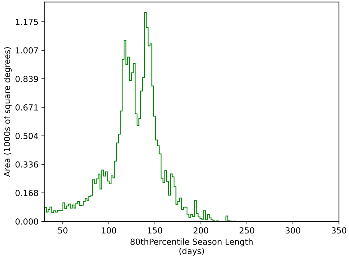
ddf_acor_sf20_lsf40_lsr50_v3.4_10yrs All sky g band: 80thPercentile Season Length
