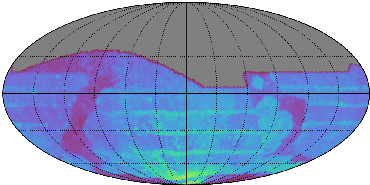
ddf_acor_sf20_lsf40_lsr50_v3.4_10yrs All sky all bands: 80thPercentile Season Length
